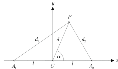
Figure 3. Two-dimensional Combined TDoA/AoA Positioning with two fixed stations (Du and Chen, 2020).
