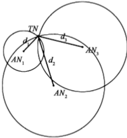
Figure 1. Two-dimensional ToA Positioning System with three fixed anchors (Liu et al. , 2007).
