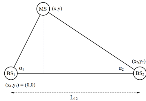
Figure 2. AoA Positioning with two fixed stations (Stan and John, 2003).
