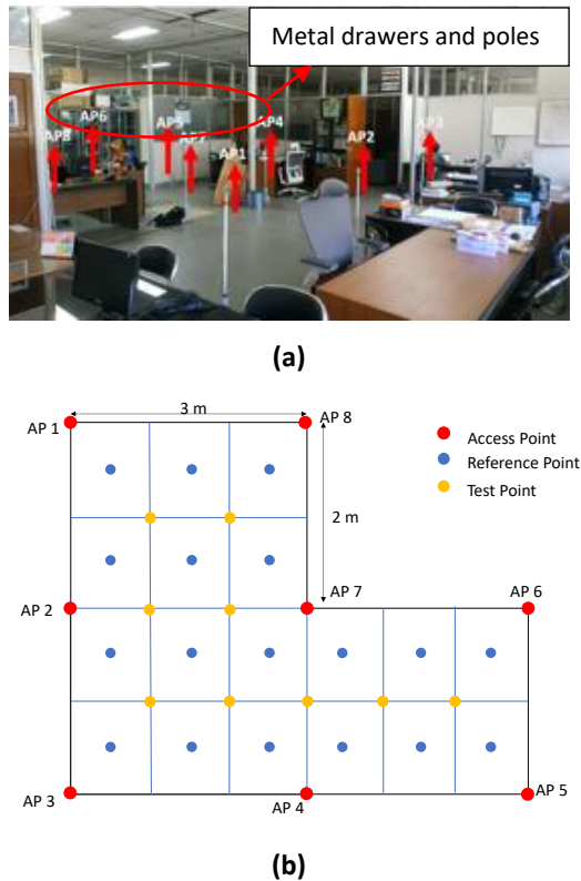
Figure 6. Measurement scenarios (a) APs locations (b) Testing positions outside fingerprint location
