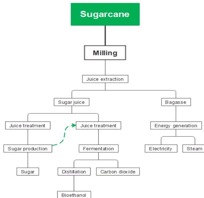
Figure 2. Bioethanol production from sugarcane
