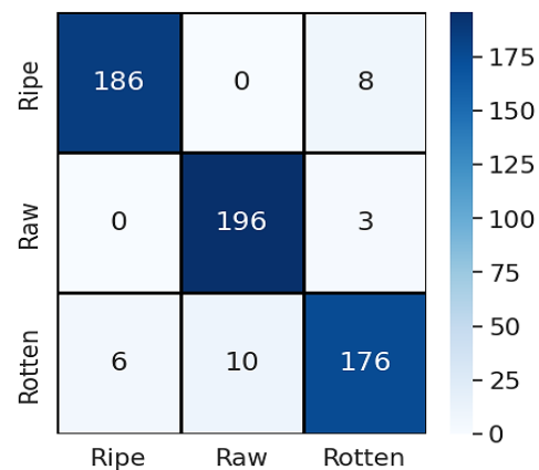
Figure 7. Confusion matrix measurement
