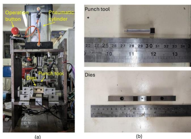
Figure 3. (a) micro punch machine, and (b) tools and dies used
