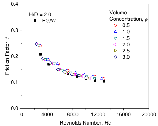
Figure 11. Friction factor of ternary nanofluids with twisted tape for H/D = 2.0
